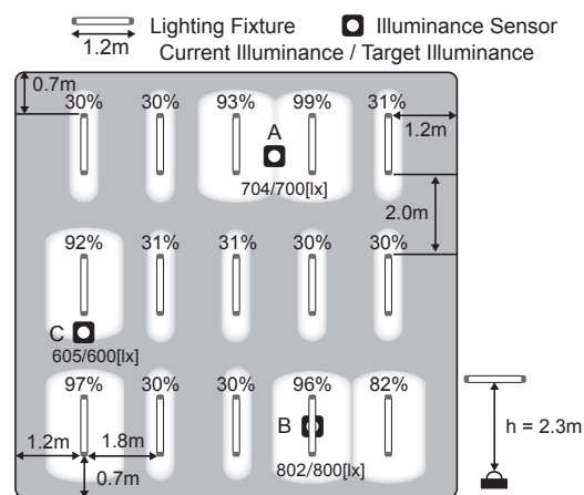
Fig. 1. Lighting pattern resulting in the Intelligent Lighting System.
