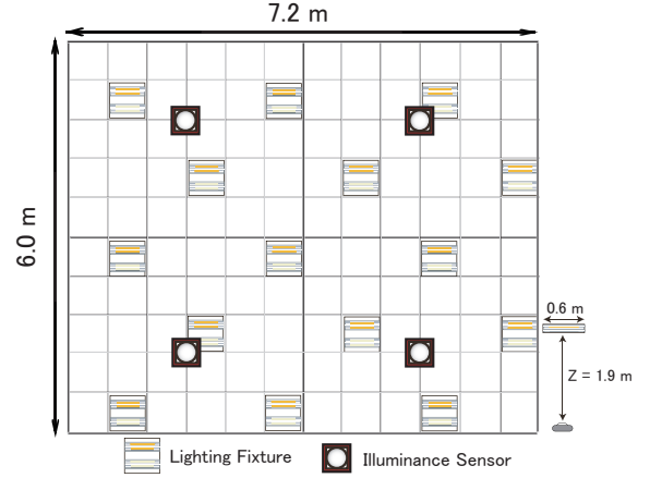
Fig. 2. Experimental environment to obtain regression coefficients
