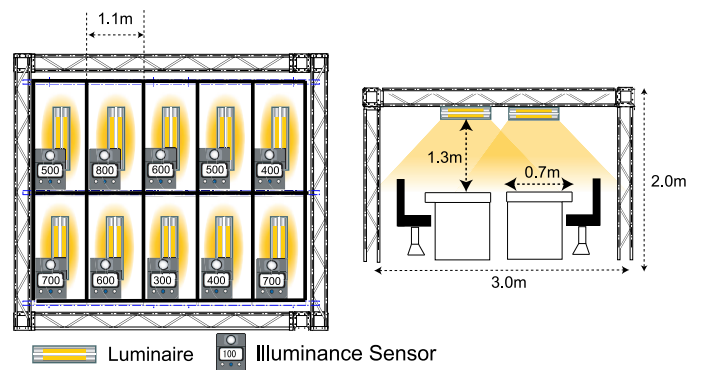
Fig. 12. Experiment institution at actual workspace
