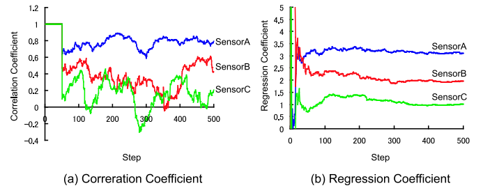
Fig. 7. History of the factor of influence
