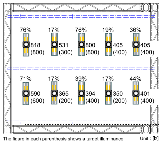
Fig. 13. Distribution of the luminance and illuminance
