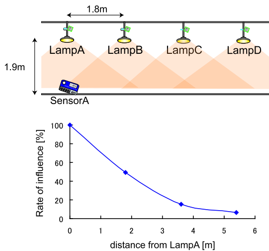
Fig. 8. Relation between position and influence
