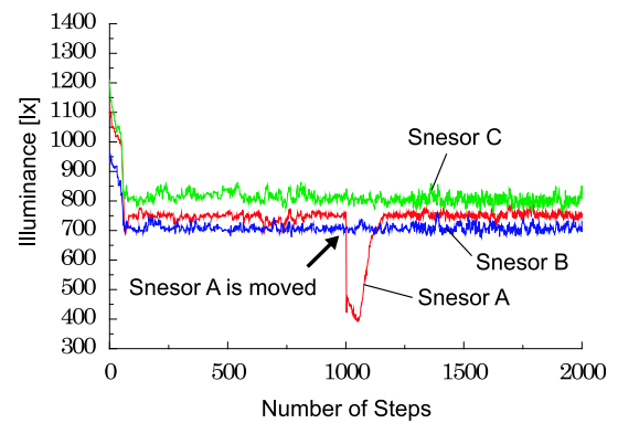
Fig. 4. History of illuminance(ANA/CC)
