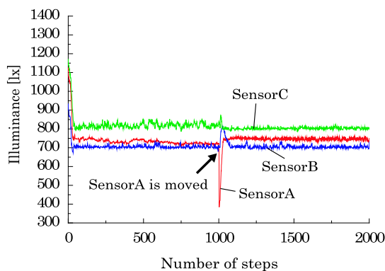
Fig. 10. History of illuminance(ANA/RC)
