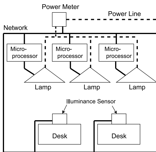
Fig. 1. Configuration of Intelligent Lighting System
