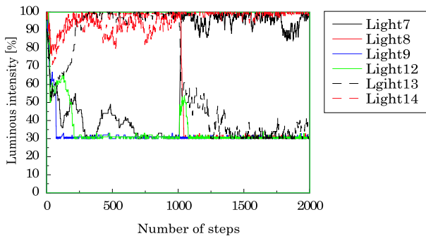
Fig. 11. History of luminance(ANA/RC)
